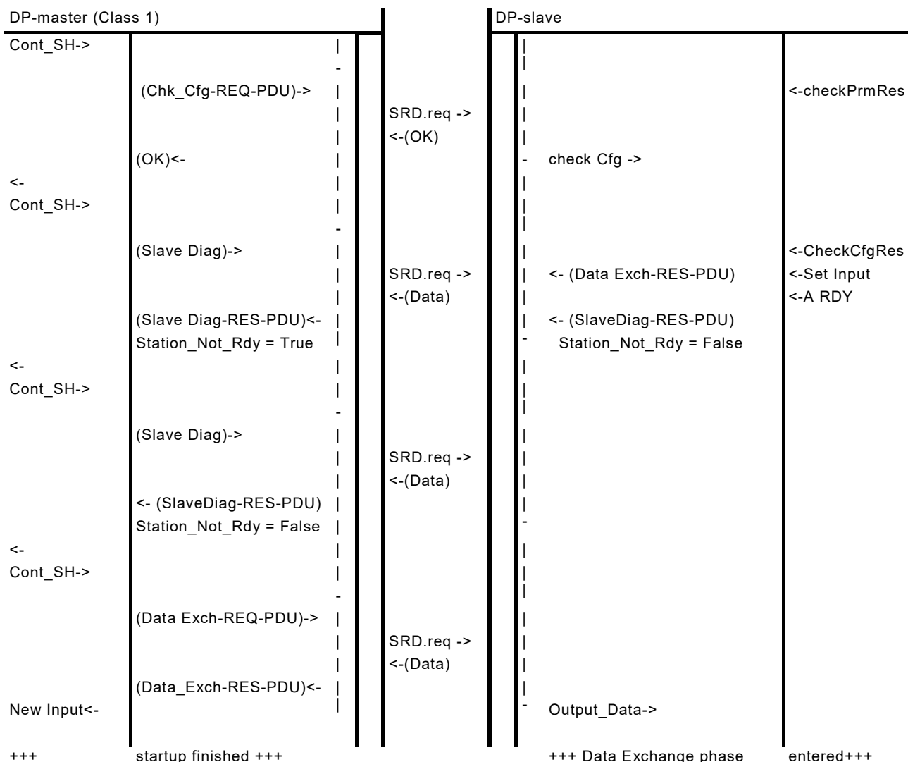
Figure 16 – Sequence of the communication between DP-master and DP-slave
