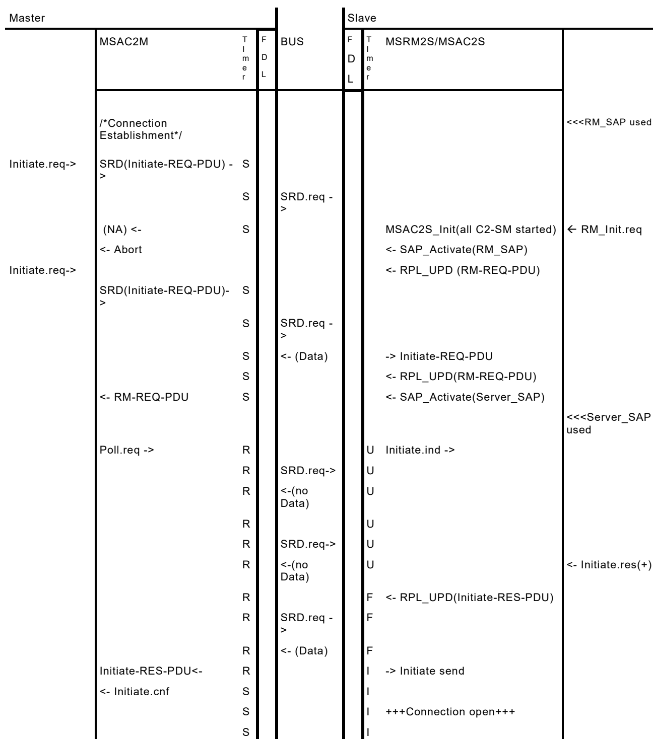
Figure 19 – Example for connection establishment on MS2
